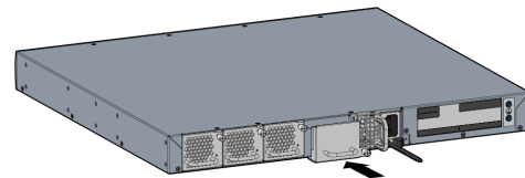
Figure 2 Installing a Filler Panel
